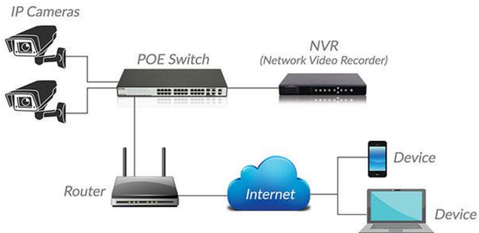
CCTV IP Cameras with Local NVR Storage
